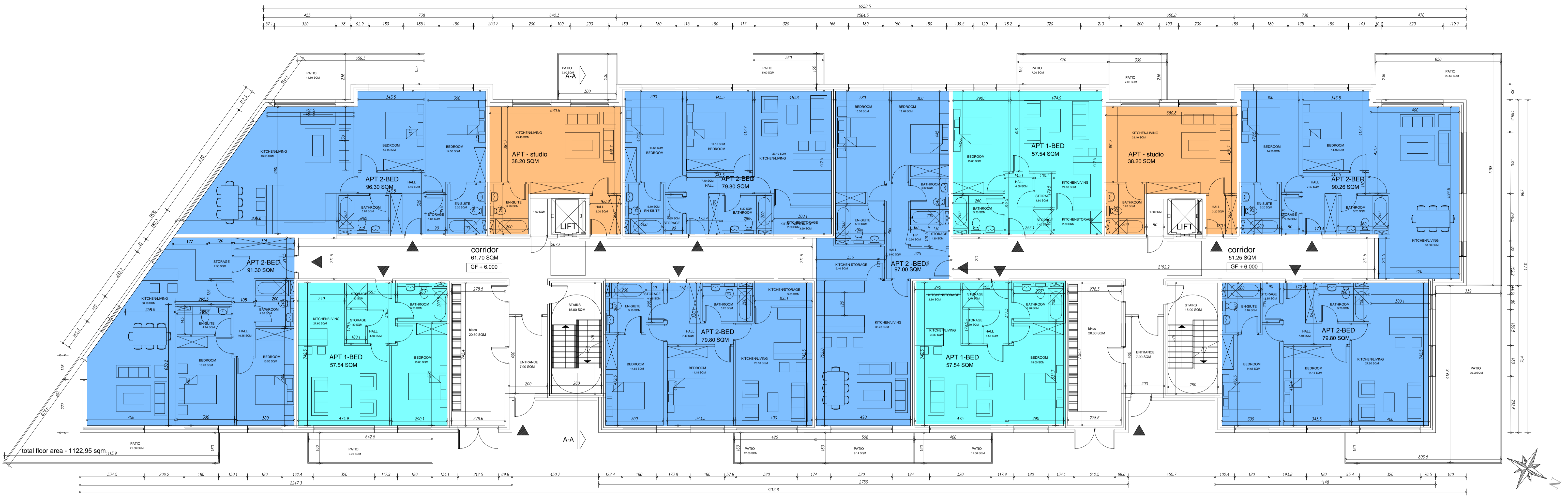
1 PROPOSED BLOCK 3 - GROUND FLOOR PLAN
